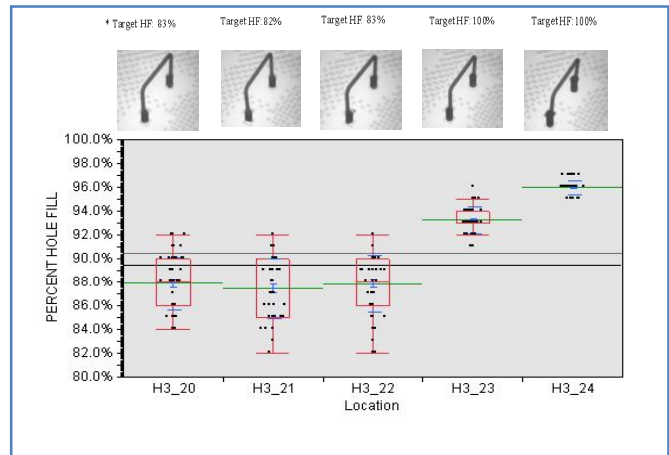
Figure 6.6: Box plot of holefill% for different combination of solder preforms. A sample x-ray image and target holefill% for each case, are shown at top of the box plot.
