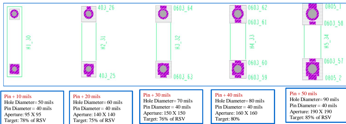
Figure 3.5: Effect of Pin to Hole Clearances
