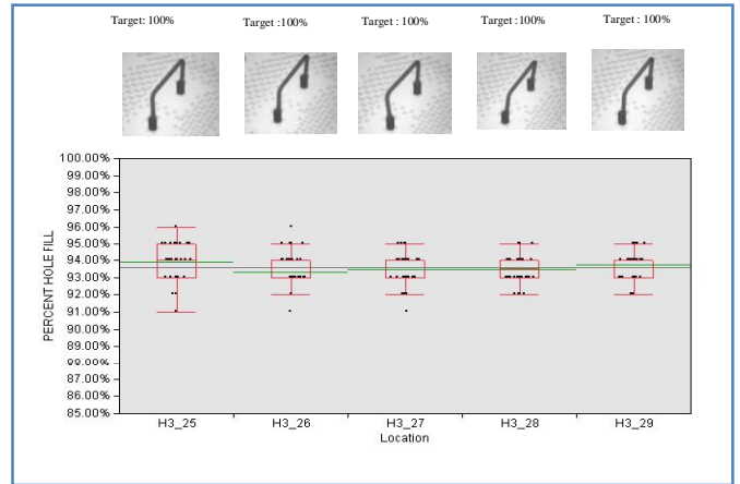
Figure 6.8: Box plot of holefill% for solder preforms placed at different locations within the solder paste.
