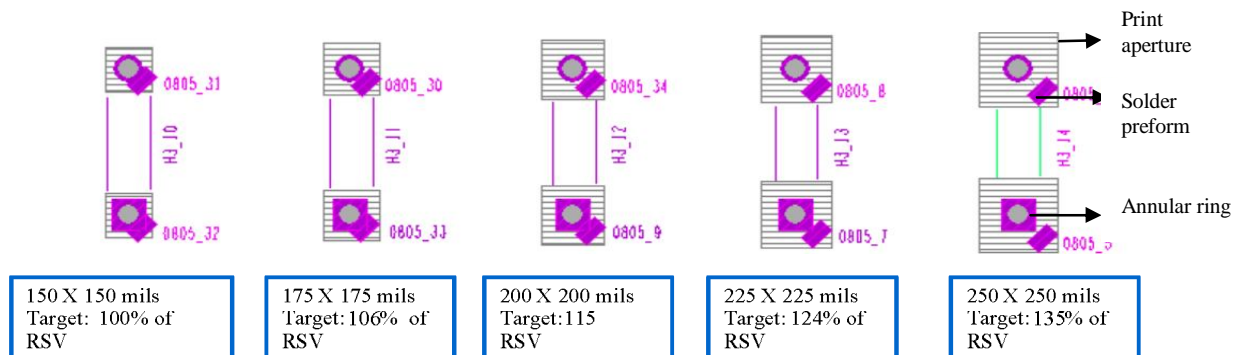
Figure 3.1: Overprinting around annular ring with 0805 preform at corner. The worst case scenario is 250 X 250 mils. A 2 pin staple was used to study the problem. The pin has square pad on one end and circular pad on other end
