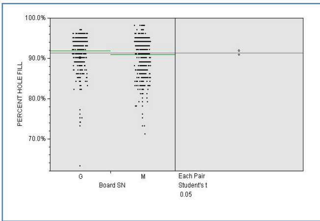
Figure 6.3: Box plot of holefill% comparing glossy and matte solder masks. Paired t-test shows no significant difference.
