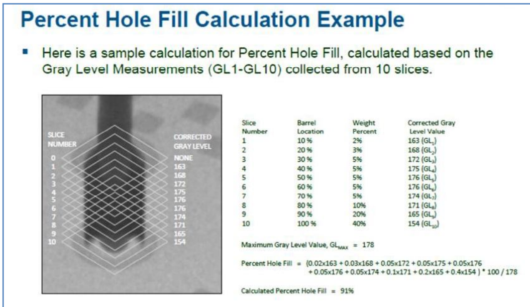
Figure 5: Sample Holefill Calculation using 5DX Equipment
