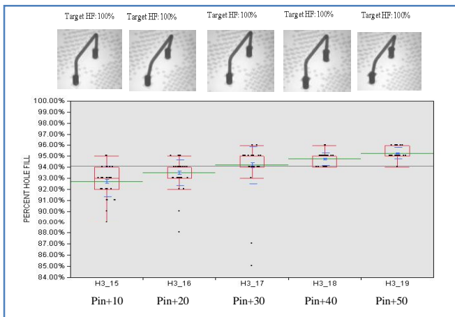
Figure 6.5: Box plot of holefill% for solder paste overprinting with offset. A sample x-ray image and target holefill% for each case, are shown at top of the box plot.
