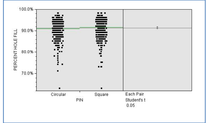
Figure 6.2: Box plot of holefill% comparing circular and square annular ring pads. Paired t-test shows no significant difference
