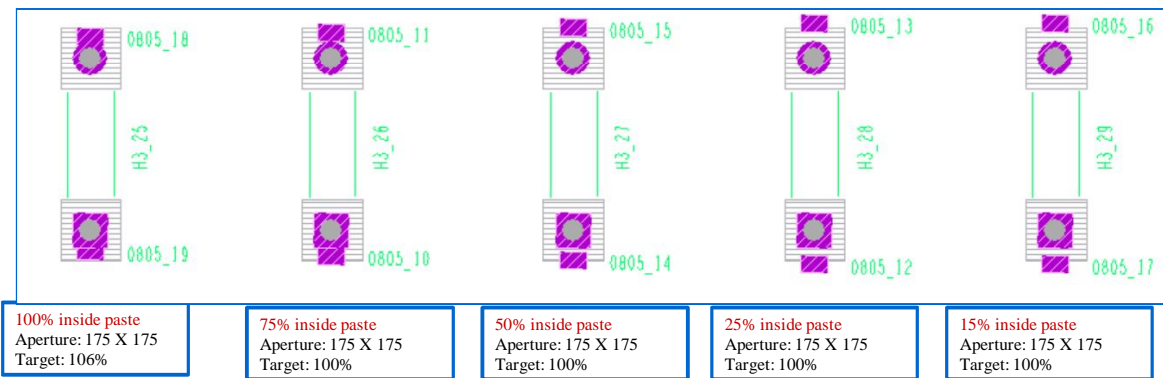
Figure 3.4: Limitation of Placing Preforms within the solder pastes
