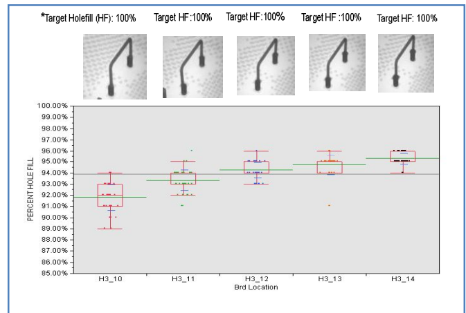
Figure 6.4: Box plot of holefill% for solder paste overprinting. A sample x-ray image and target holefill% for each case, are shown at top of the box plot.
