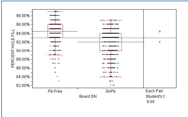
Figure 6.1: Box plot of holefill% comparing tin-lead and lead-free assembly. Paired t-test shows no significant difference.
